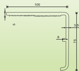
100mm lengthening corn frame
